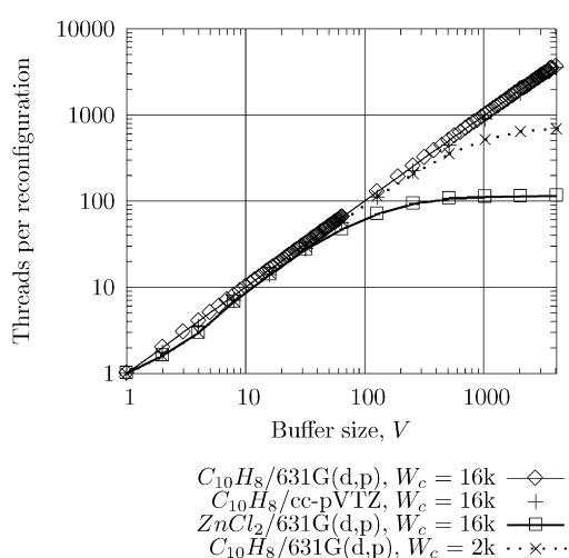
Fig. 5. FPGA ERI pipeline reconfigurations vs. V .
