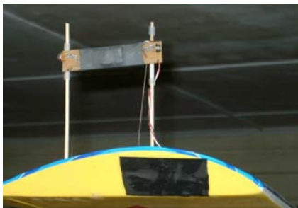
Figure 11. Movable pitch sensor controlled by a servo under the black tape..
