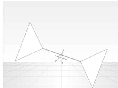
Figure 5. Fixed wingtip roll sensors
