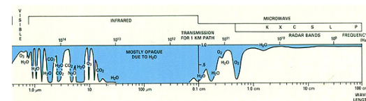
Figure 1. Useful atmospheric windows
