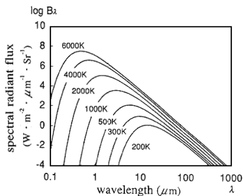
Planck's Law Figure 3.
