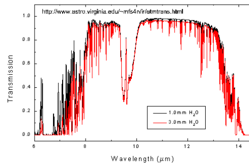
Figure 2. Thermal or mid infrared window with effects of precipitable water vapour
